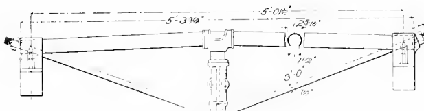
Figs. 4899. Plan. UNIVERSAL BRAKE-BEAM.
